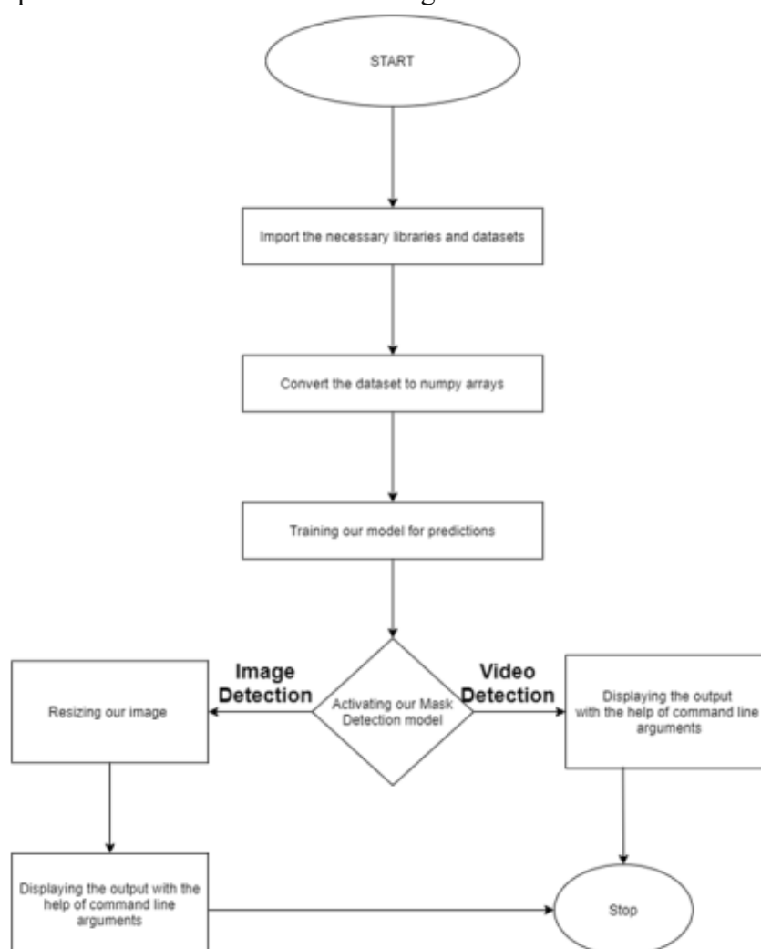
Figure 2: Flowchart for face-mask detection
