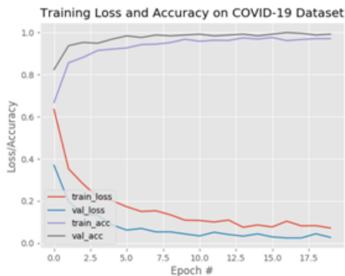
Figure 6: The accuracy of the aforementioned model
